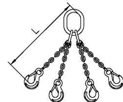
4-Strang-Anschlagkette
